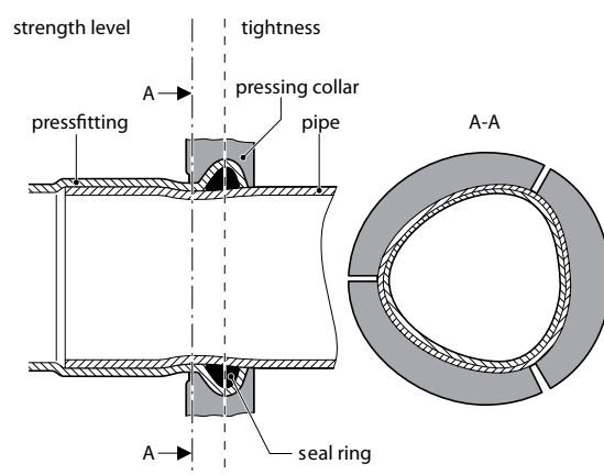
Figure 2: Section through a pressfitting joint with the pressing collar (lemon shaped pressing contour) still in position.
